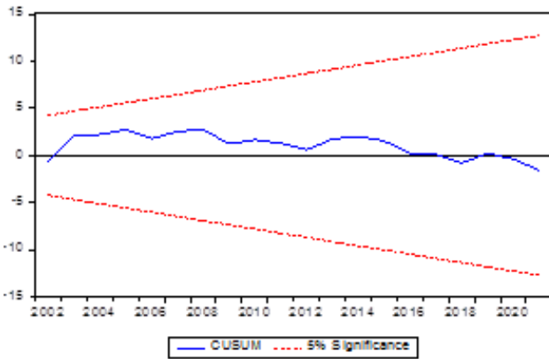
Figure 3. Plot of CUSUM.
