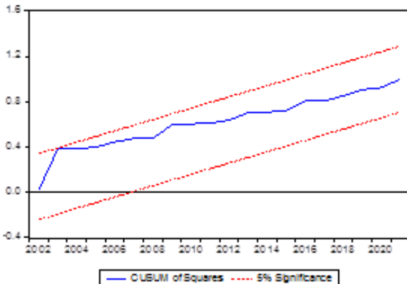
Figure 4. Plot of CUSUMSQ.
